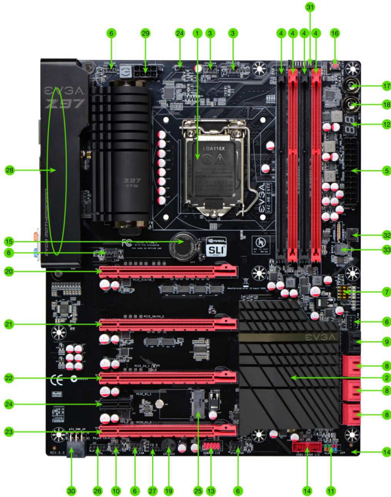
FIGURE 1. Z97 FTW Motherboard Layout
