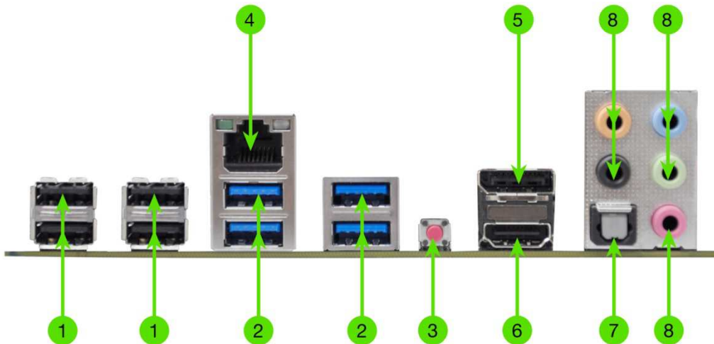
Figure 2. Chassis Rear Panel Connectors
