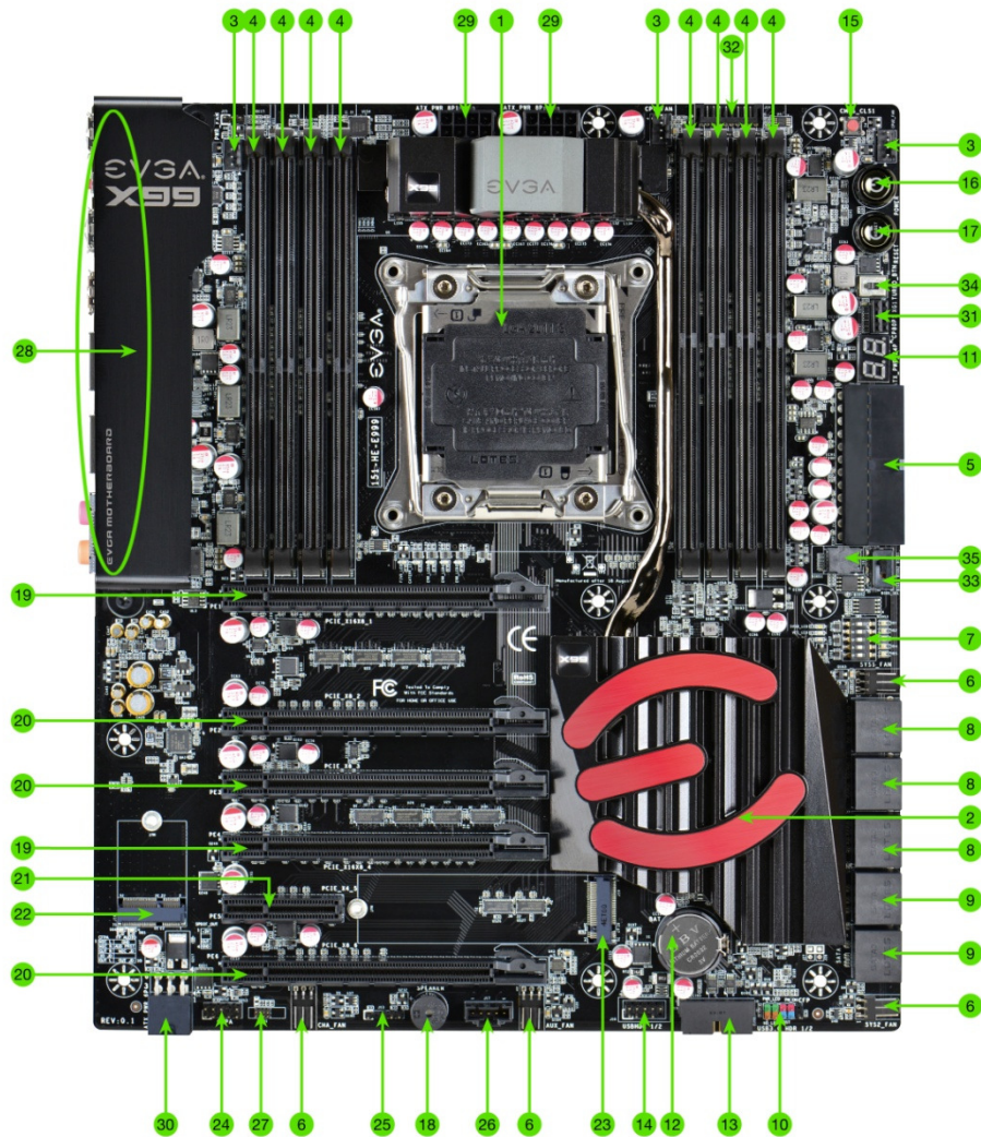
FIGURE 1. X99 Classified Motherboard Layout
