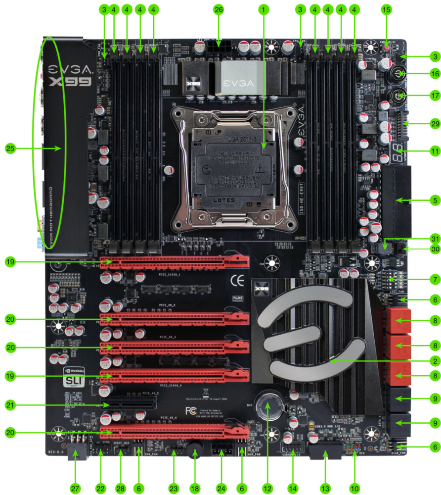
FIGURE 1. X99 FTW Motherboard Layout
