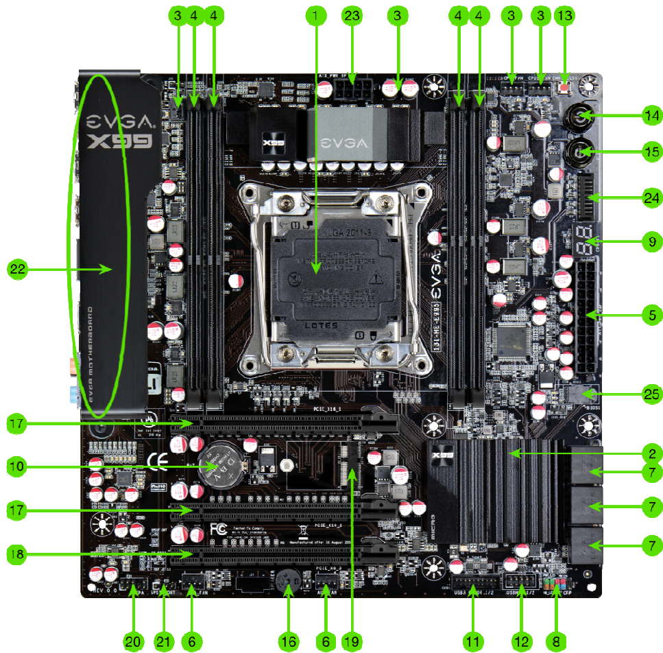
FIGURE 1. X99 Micro Motherboard Layout
