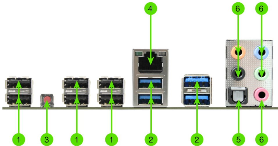
Figure 2. Chassis Rear Panel Connectors
